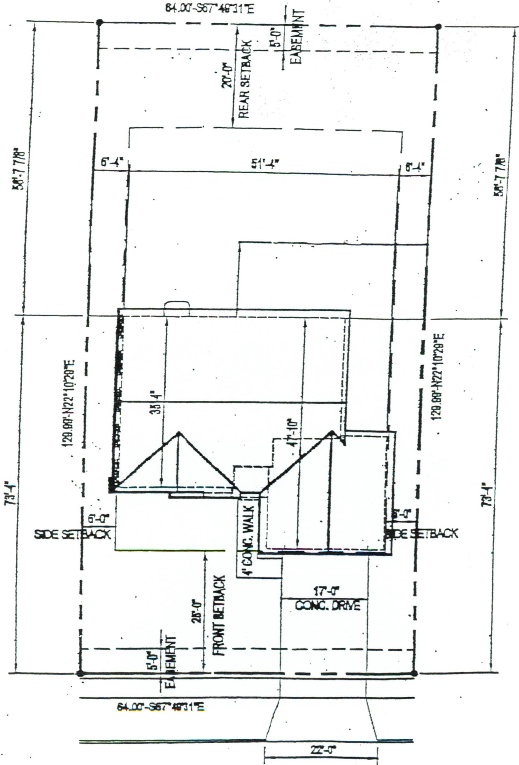
Typical illustration of a plot plan or mortgage survey
